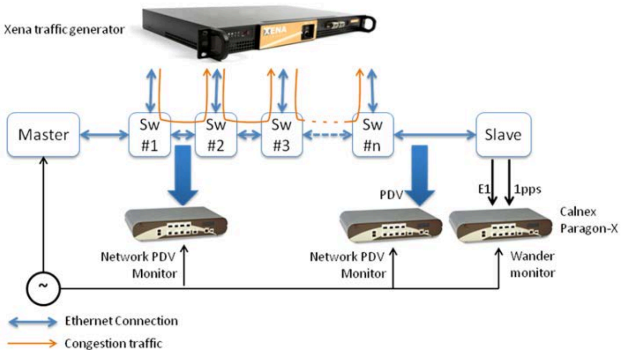
Figure 1 Generic test configuration
