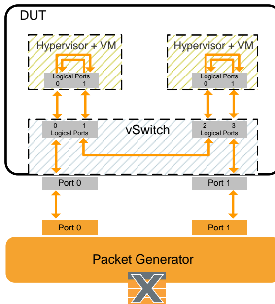
Figure 3. PVVP scenario
