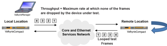
▪ Figure 3 RFC 2544 Throughput Test
