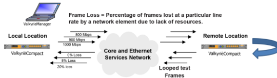
▪ Figure 4 RFC 2544 Frame Loss Test
