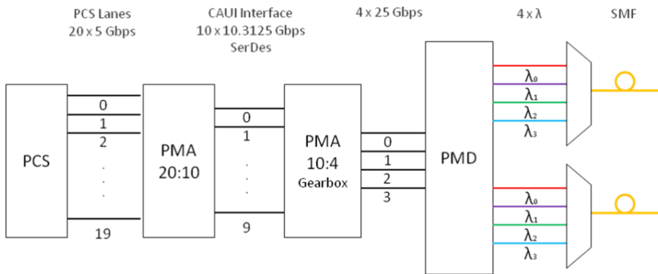
▪ Figure 2 PHY (PCS and PMA) for 100G CAUI with LR4 optical transceiver
