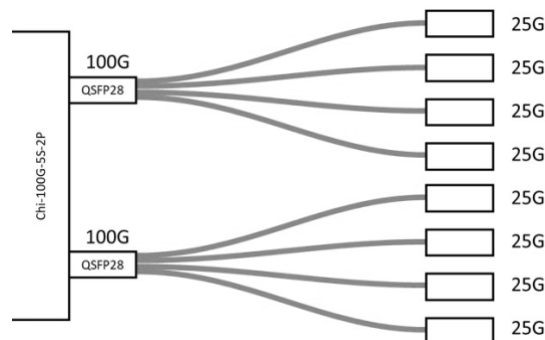
Figure 13: Break-ou1 from two 100G ports to eight 25G ports.
