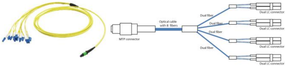
Figure 7: MTP to 4 dual LC passive optical splitter cable
