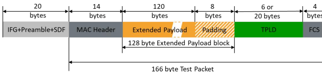
Figure 16: Test packet with 120 bytes Extended Payload
