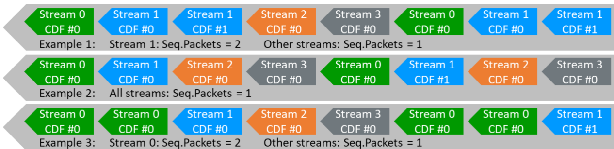
Figure 11: Sequential test packet flow examples with different Seq.Packets settings
