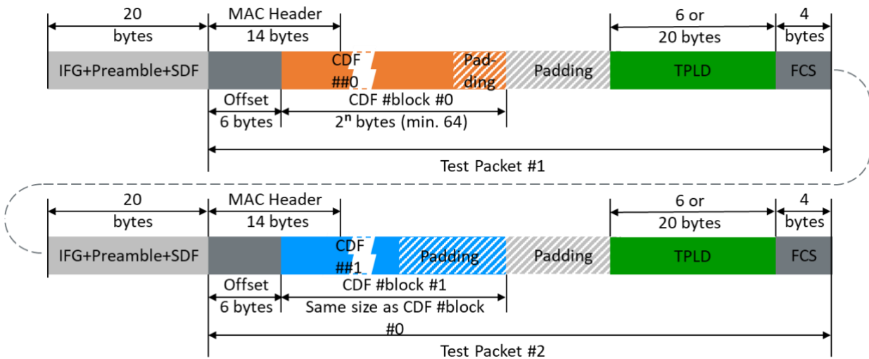
Figure 2: Stream definition with two CDFs overwriting a part of the MAC header
