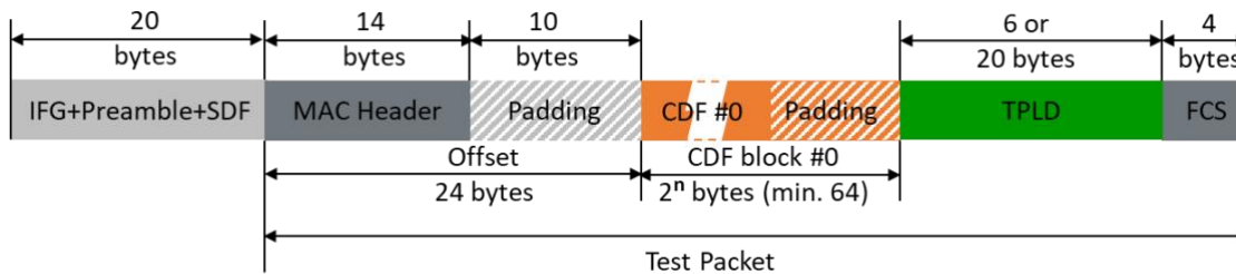
Figure 3: Test packet with one CDF, starting 10 bytes after the protocol header (in this case a MAC header)
