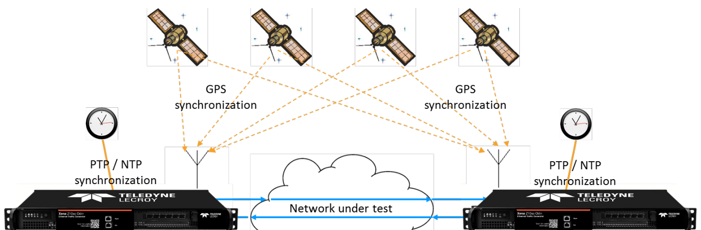
Figure 2: WAN scenario: Test chassis synchronize time using GPS signals and/or NTP/PTP servers
