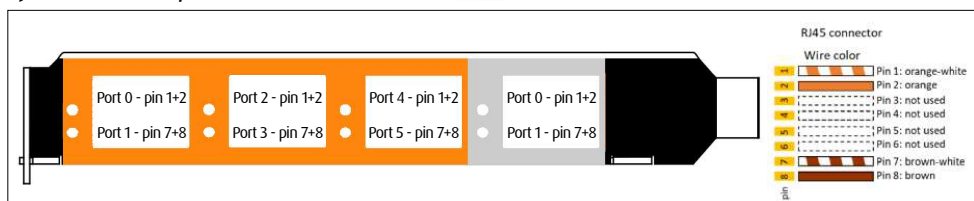
RJ45 connector pin out:
